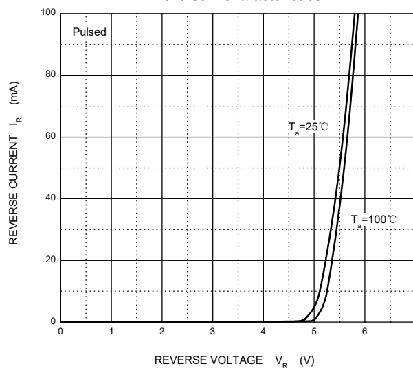
Reverse Characteristics
